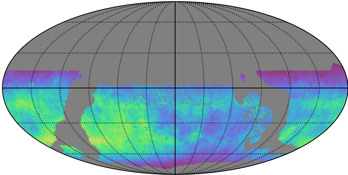
too_elab_r64_d3_giz_v3.4_10yrs WFD z band: Normalized Teff
