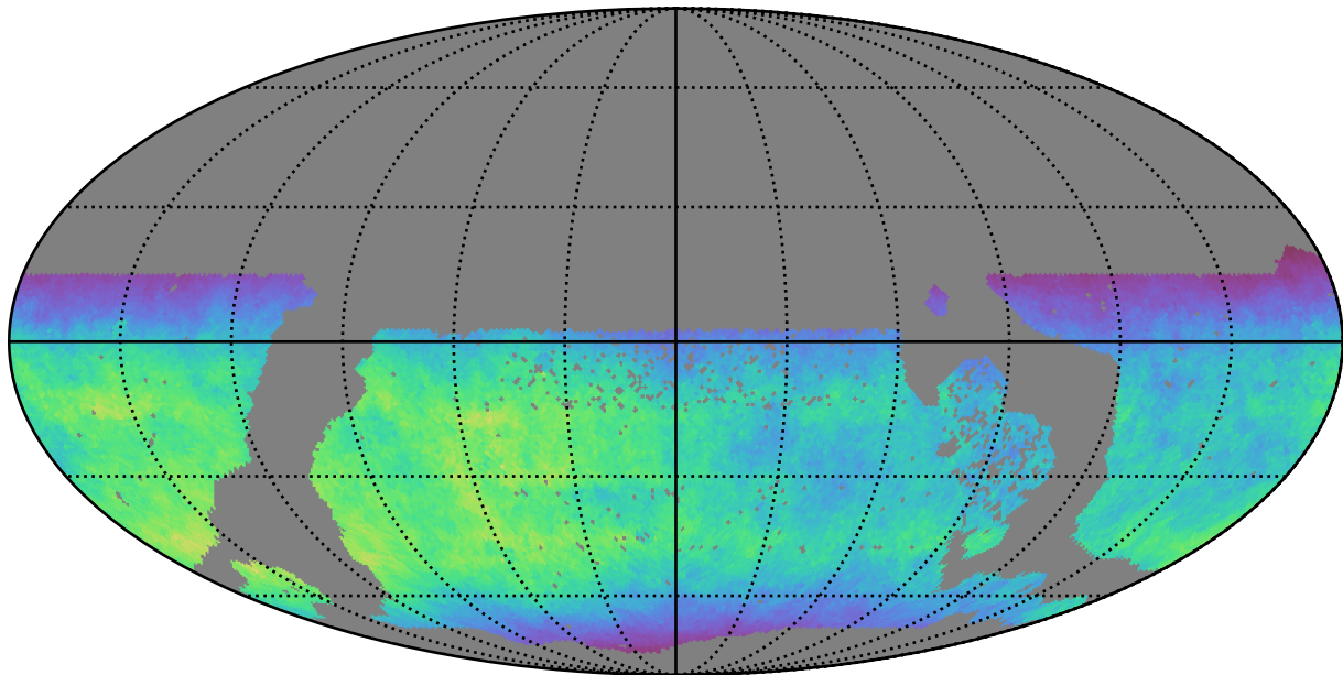
too_elab_r64_d3_giz_v3.4_10yrs WFD y band: Normalized Teff
