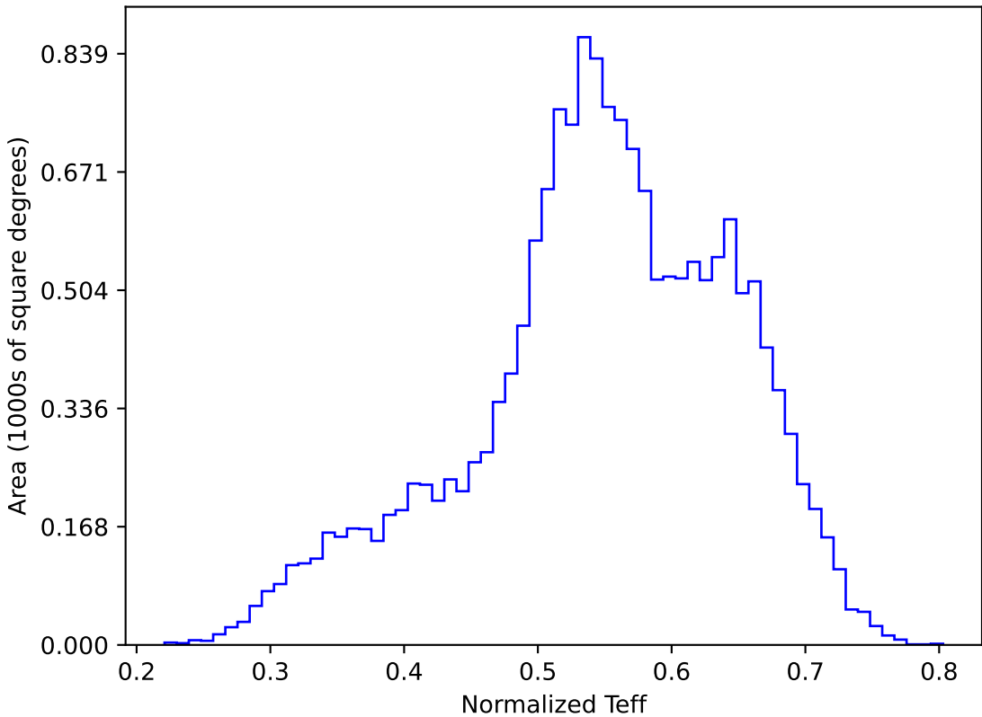
too_elab_r64_d3_giz_v3.4_10yrs WFD y band: Normalized Teff
