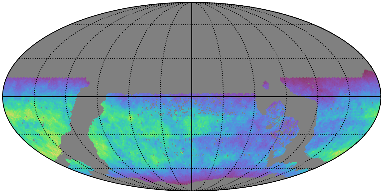
too_elab_r64_d3_giz_v3.4_10yrs WFD u band: Normalized Teff
