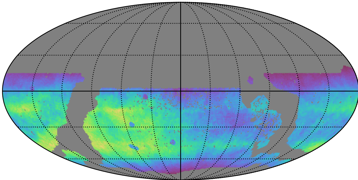
too_elab_r64_d3_giz_v3.4_10yrs WFD r band: Normalized Teff
