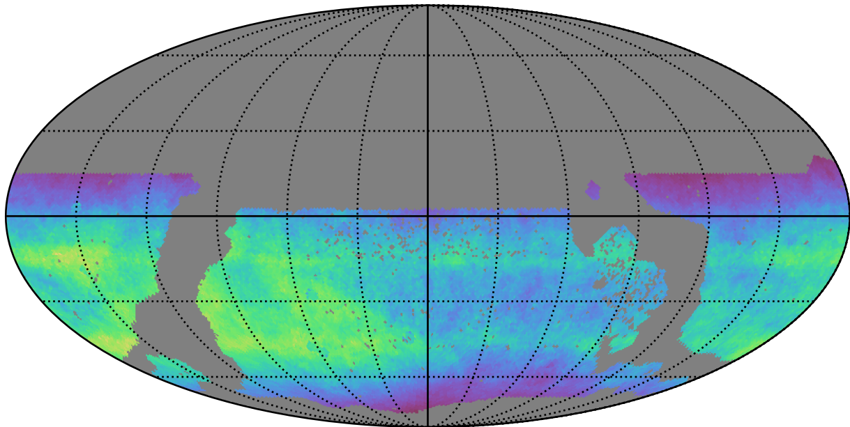
too_elab_r64_d3_giz_v3.4_10yrs WFD i band: Normalized Teff
