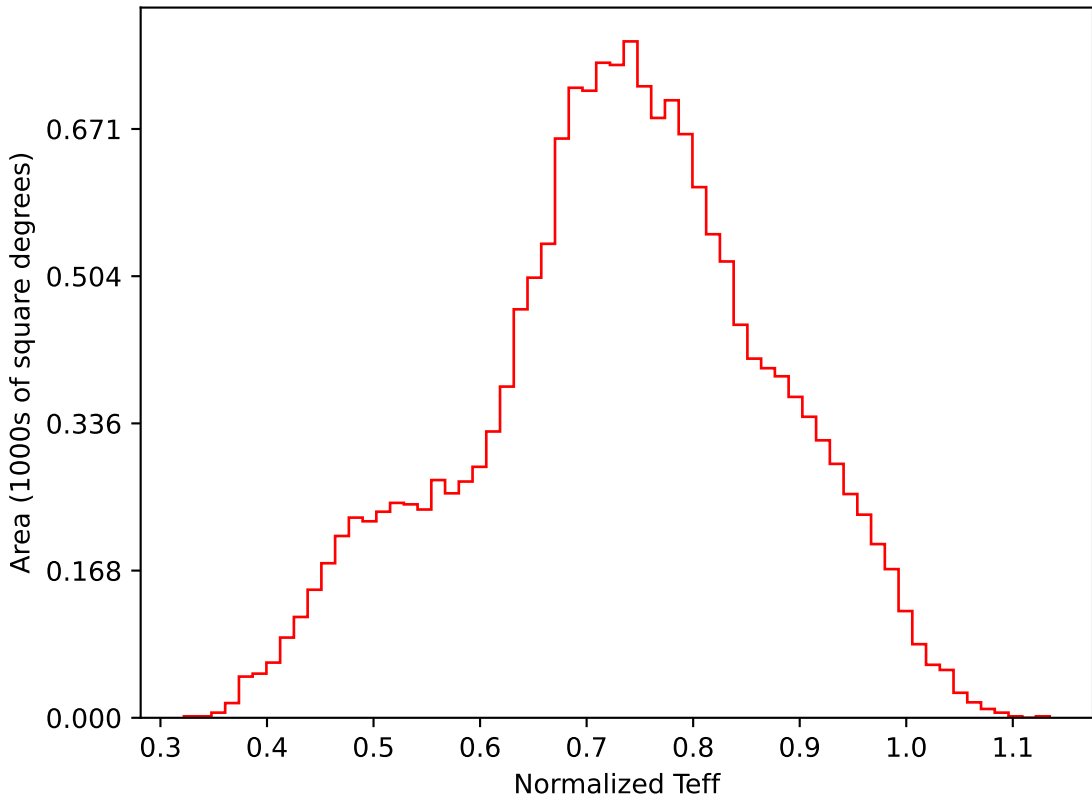
too_elab_r64_d3_giz_v3.4_10yrs WFD i band: Normalized Teff
