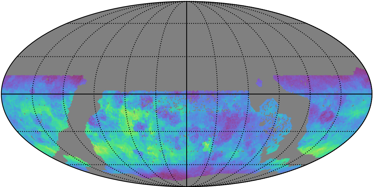
too_elab_r64_d3_giz_v3.4_10yrs WFD g band: Normalized Teff
