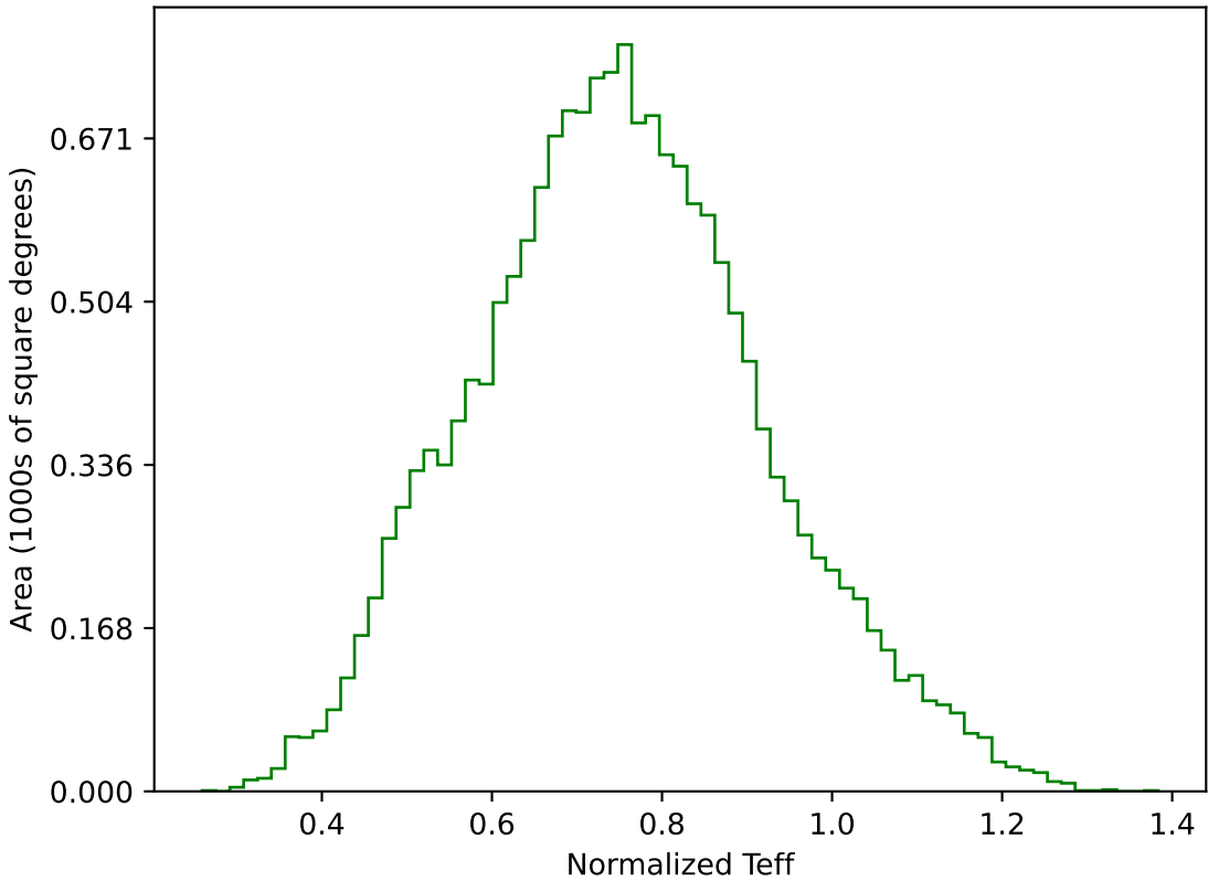
too_elab_r64_d3_giz_v3.4_10yrs WFD g band: Normalized Teff
