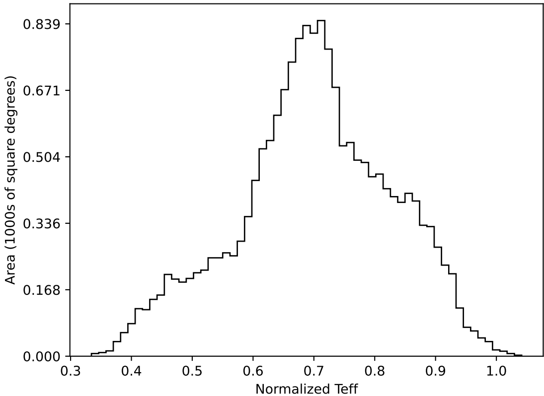
too_elab_r64_d3_giz_v3.4_10yrs WFD all bands: Normalized Teff
