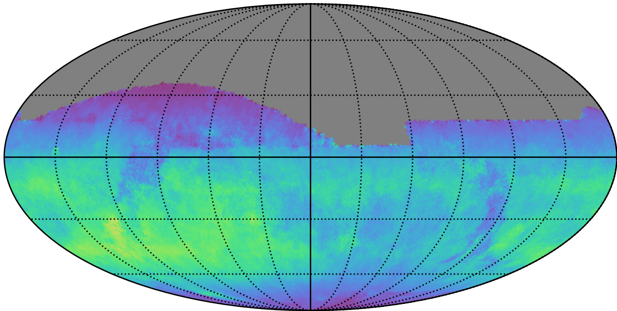
too_elab_r64_d3_giz_v3.4_10yrs All sky z band: Normalized Teff
