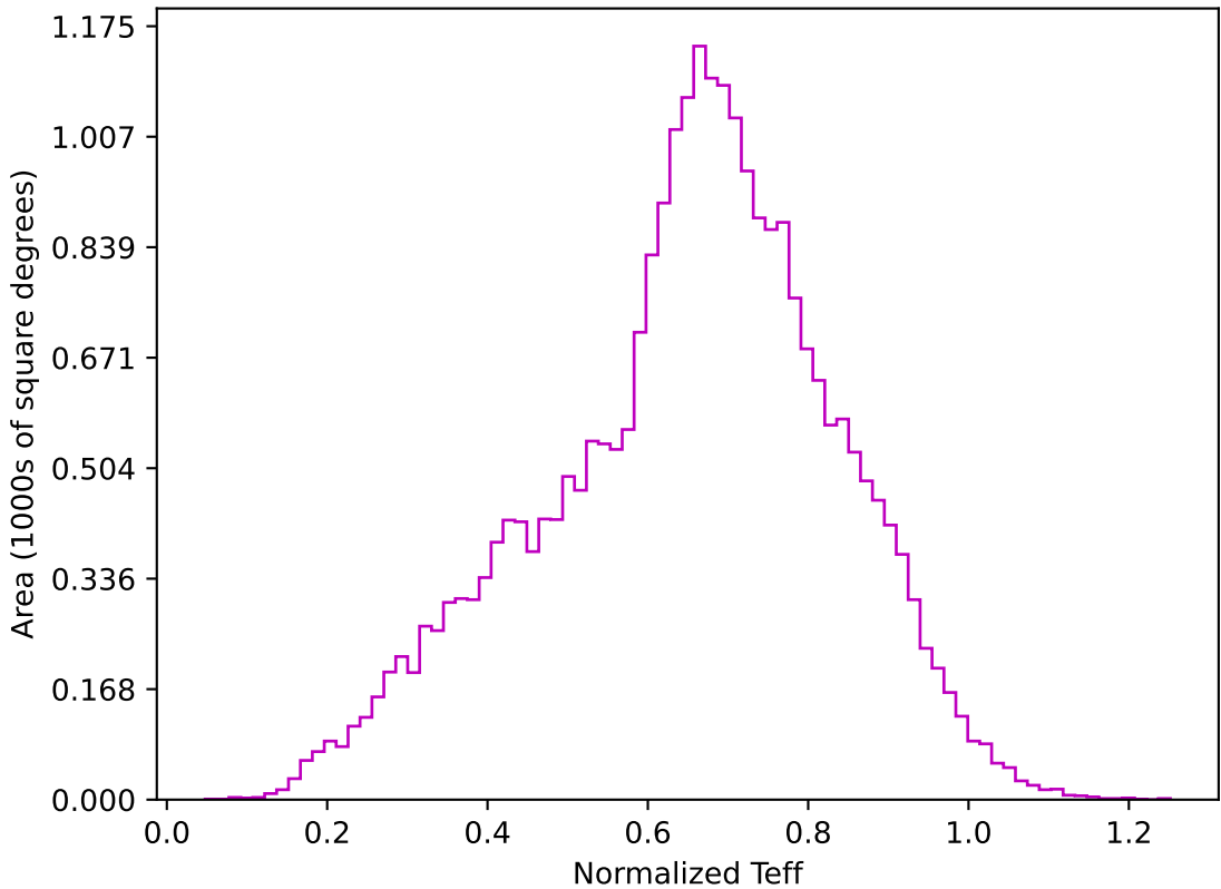
too_elab_r64_d3_giz_v3.4_10yrs All sky z band: Normalized Teff
