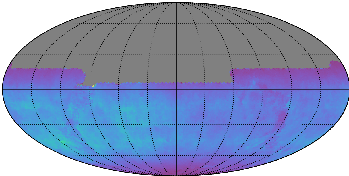
too_elab_r64_d3_giz_v3.4_10yrs All sky y band: Normalized Teff
