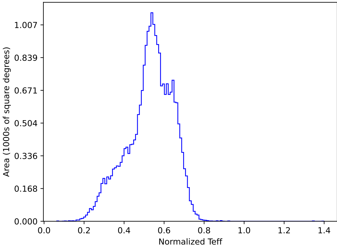
too_elab_r64_d3_giz_v3.4_10yrs All sky y band: Normalized Teff
