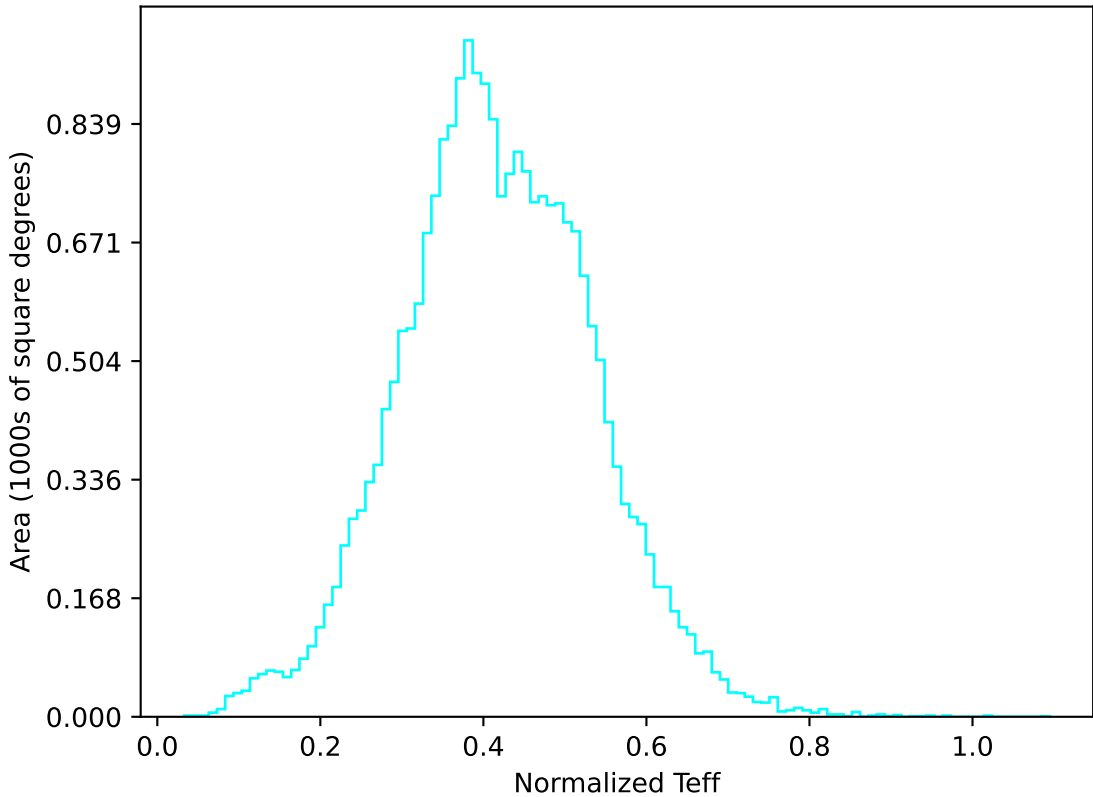
too_elab_r64_d3_giz_v3.4_10yrs All sky u band: Normalized Teff
