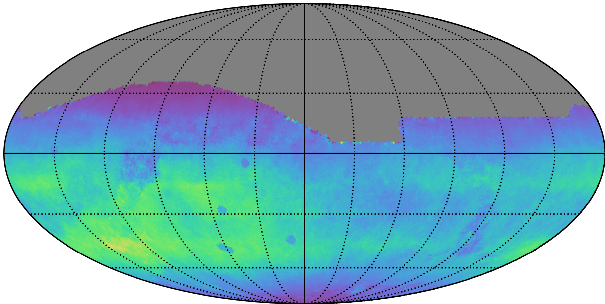
too_elab_r64_d3_giz_v3.4_10yrs All sky r band: Normalized Teff
