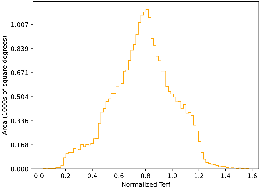
too_elab_r64_d3_giz_v3.4_10yrs All sky r band: Normalized Teff
