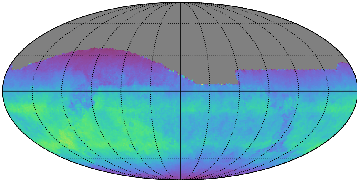
too_elab_r64_d3_giz_v3.4_10yrs All sky i band: Normalized Teff
