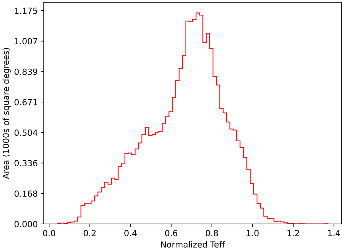
too_elab_r64_d3_giz_v3.4_10yrs All sky i band: Normalized Teff
