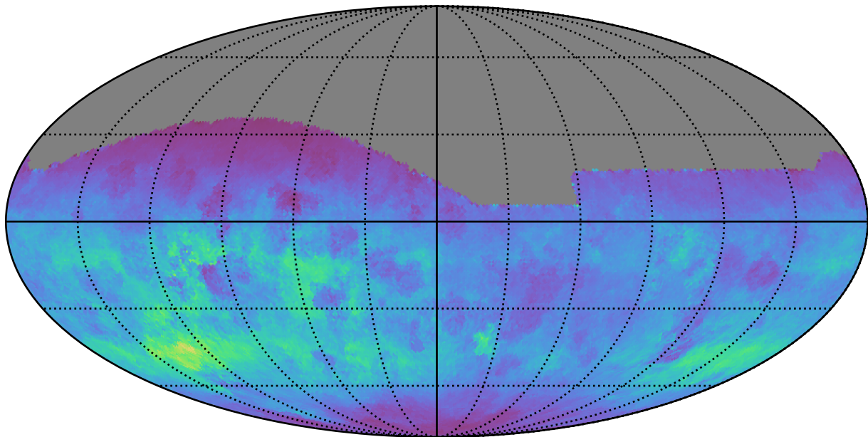
too_elab_r64_d3_giz_v3.4_10yrs All sky g band: Normalized Teff
