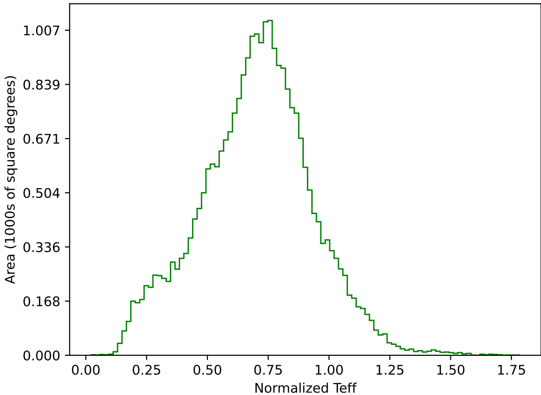
too_elab_r64_d3_giz_v3.4_10yrs All sky g band: Normalized Teff
