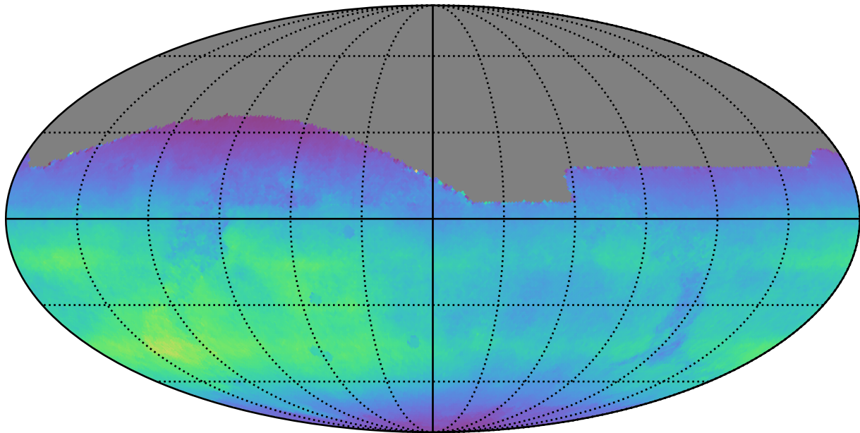
too_elab_r64_d3_giz_v3.4_10yrs All sky all bands: Normalized Teff
