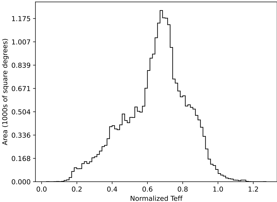
too_elab_r64_d3_giz_v3.4_10yrs All sky all bands: Normalized Teff
