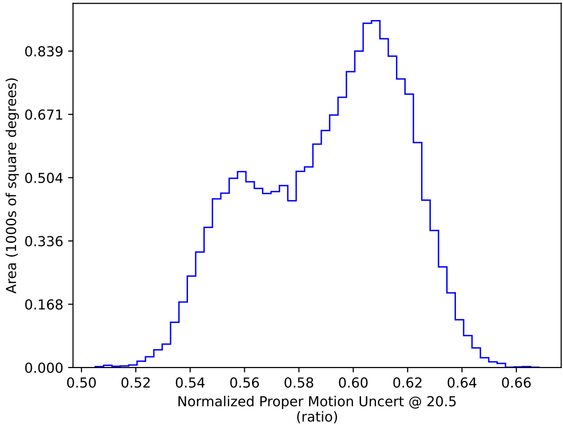
too_elab_r64_d3_giz_v3.4_10yrs WFD: Normalized Proper Motion Uncert @ 20.5
