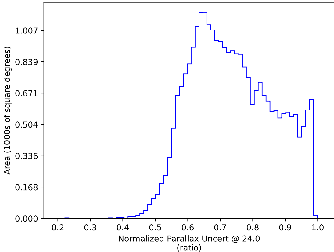
too_elab_r64_d3_giz_v3.4_10yrs All sky: Normalized Parallax Uncert @ 24.0
