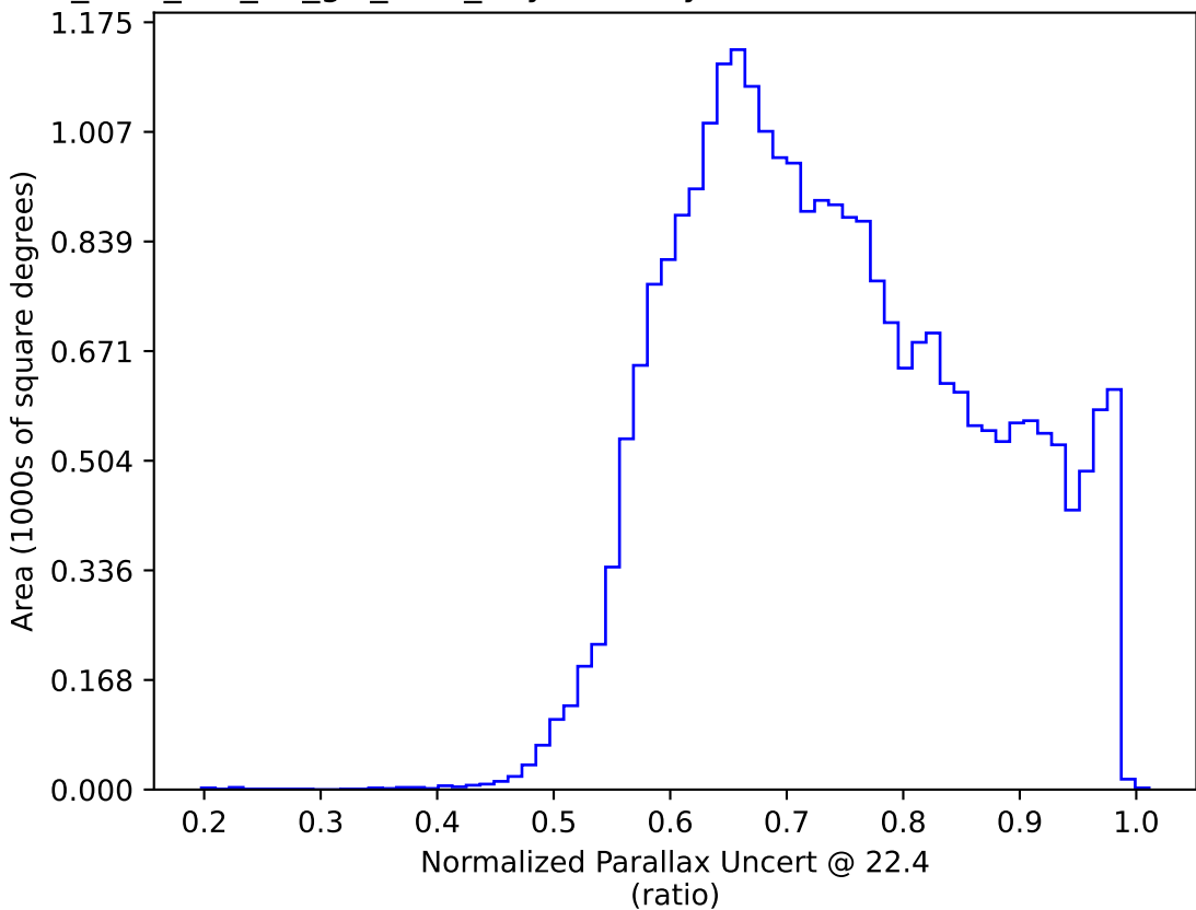
too_elab_r64_d3_giz_v3.4_10yrs All sky: Normalized Parallax Uncert @ 22.4
