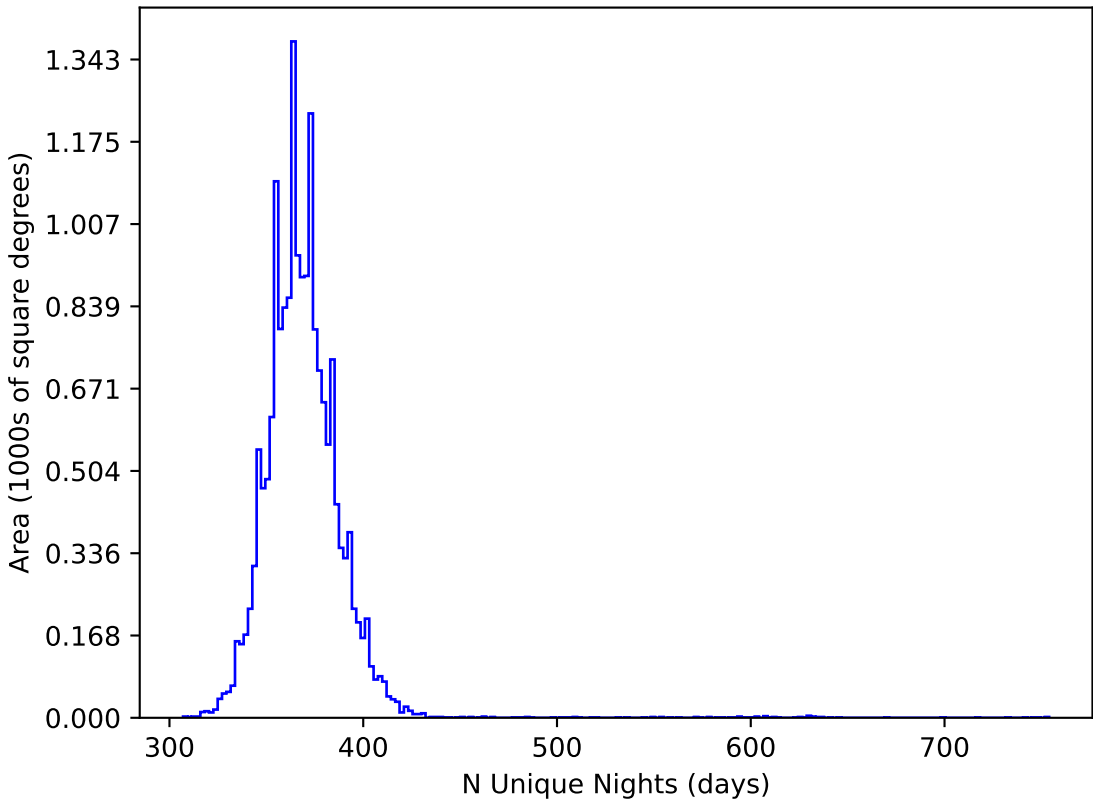
too_elab_r64_d3_giz_v3.4_10yrs WFD all bands: N Unique Nights
