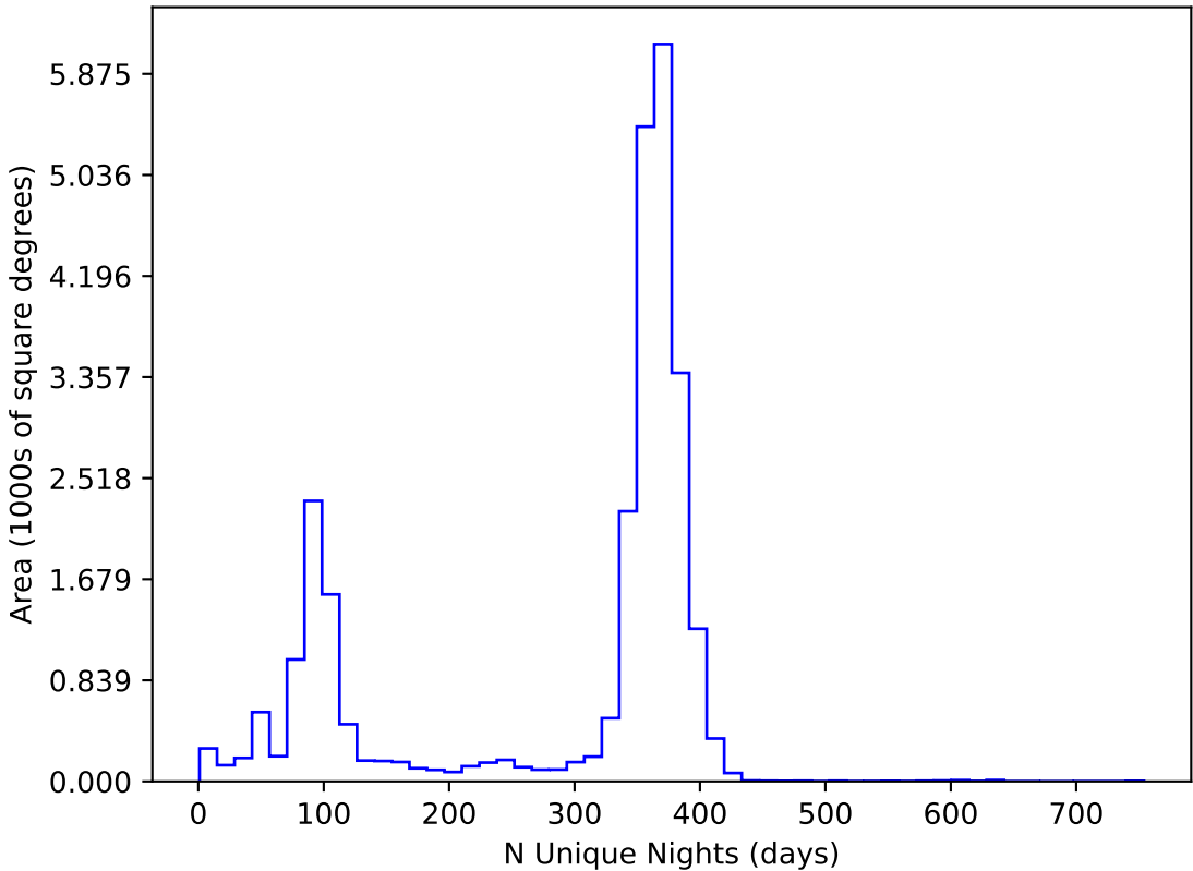
too_elab_r64_d3_giz_v3.4_10yrs All sky all bands: N Unique Nights
