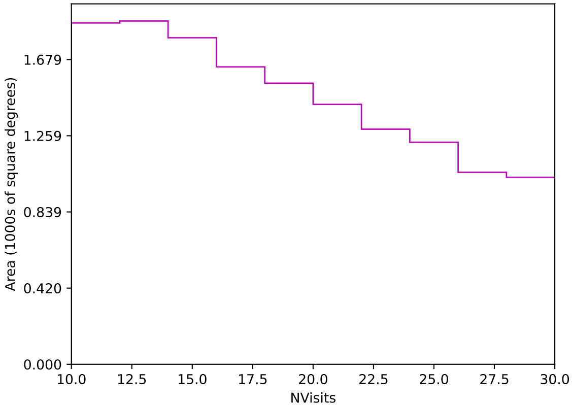
too_elab_r64_d3_giz_v3.4_10yrs Yr 3-4 z band: NVisits
