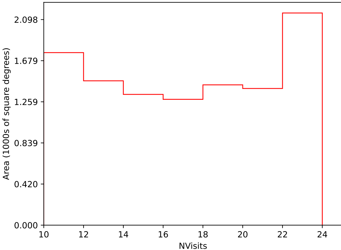
too_elab_r64_d3_giz_v3.4_10yrs Yr 3-4 i band: NVisits
