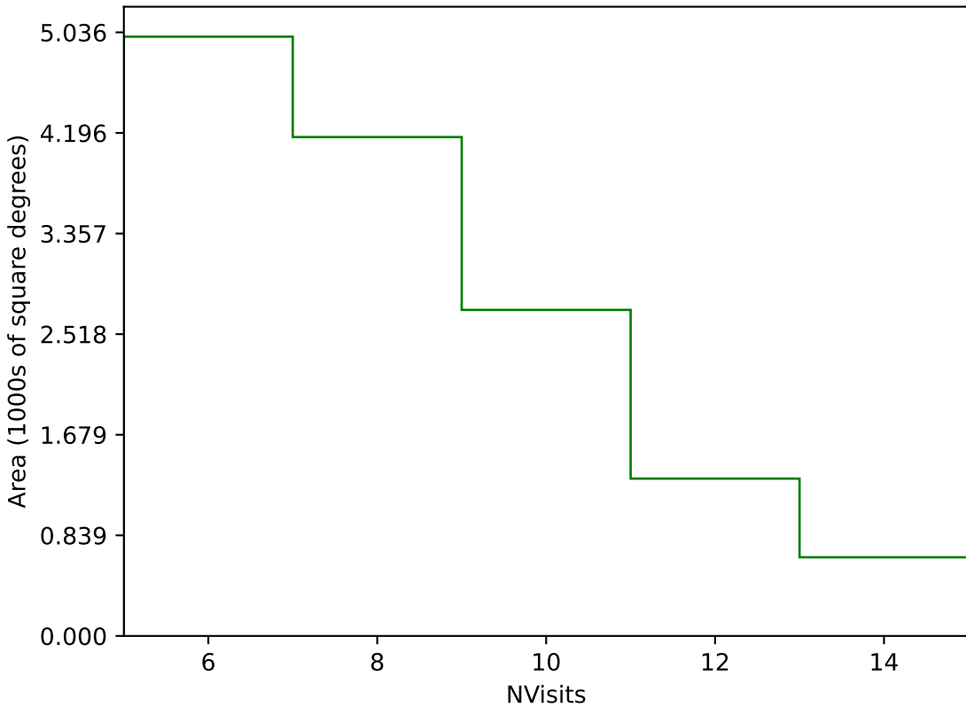
too_elab_r64_d3_giz_v3.4_10yrs Yr 3-4 g band: NVisits
