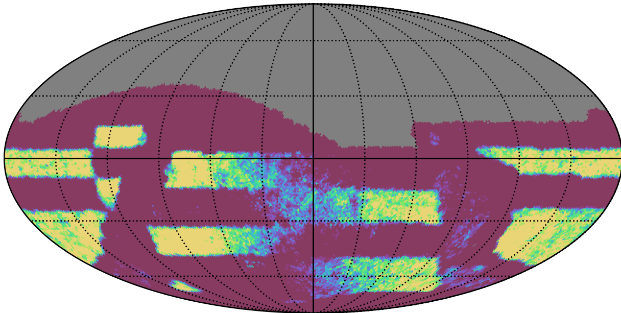
too_elab_r64_d3_giz_v3.4_10yrs Yr 3-4 all bands: NVisits
