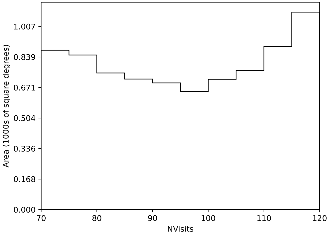
too_elab_r64_d3_giz_v3.4_10yrs Yr 3-4 all bands: NVisits
