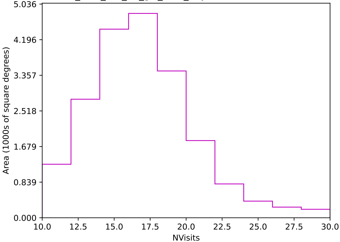
too_elab_r64_d3_giz_v3.4_10yrs Yr 1 z band: NVisits
