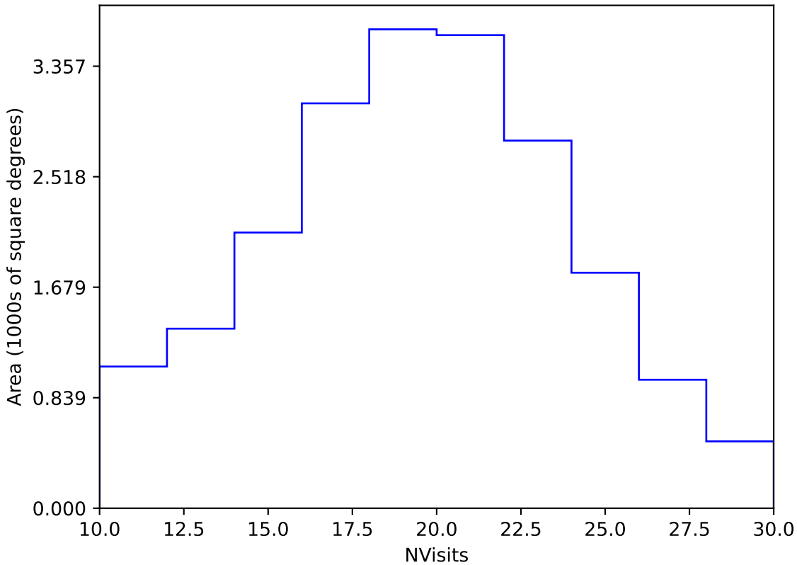
too_elab_r64_d3_giz_v3.4_10yrs Yr 1 y band: NVisits
