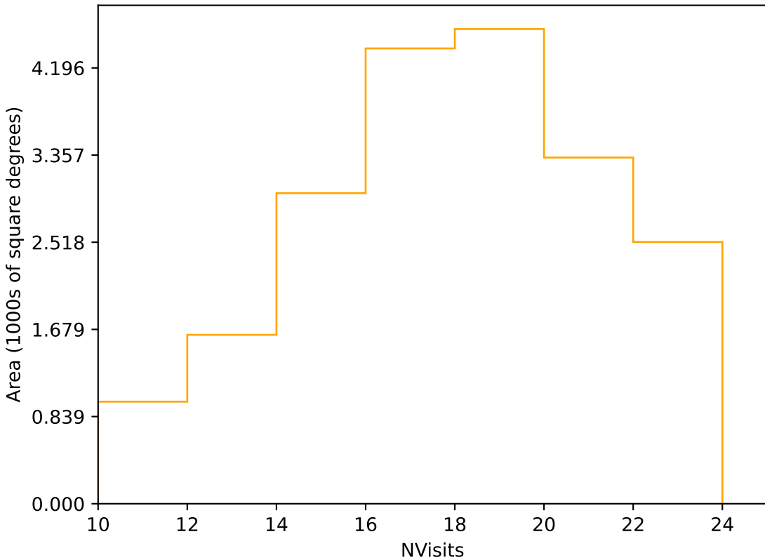
too_elab_r64_d3_giz_v3.4_10yrs Yr 1 r band: NVisits
