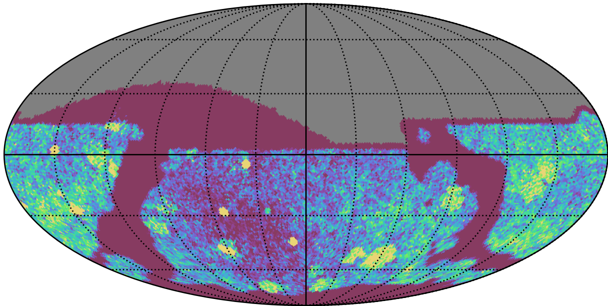
too_elab_r64_d3_giz_v3.4_10yrs Yr 1 all bands: NVisits
