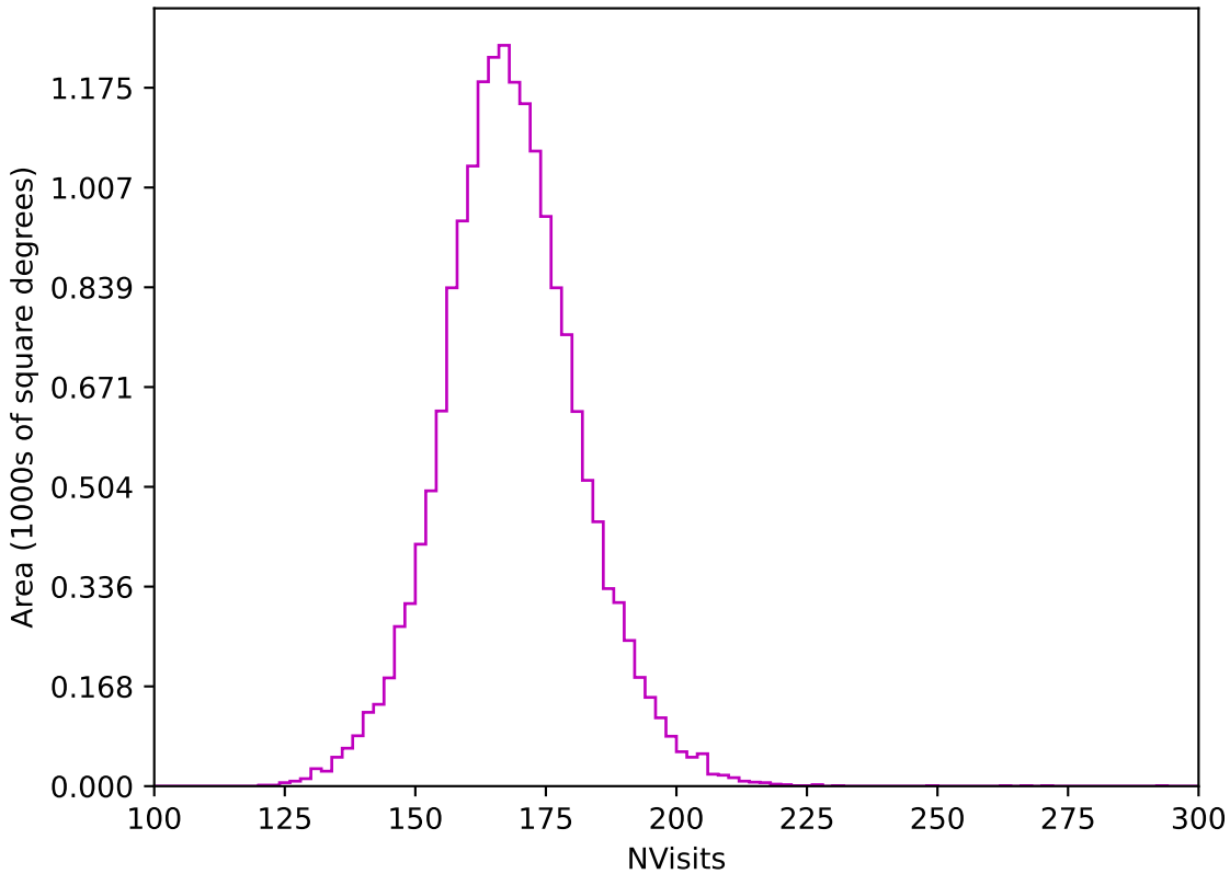
too_elab_r64_d3_giz_v3.4_10yrs WFD z band: NVisits
