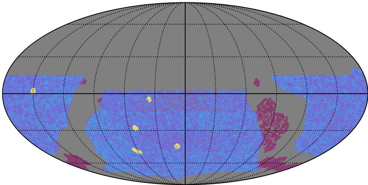
too_elab_r64_d3_giz_v3.4_10yrs WFD y band: NVisits
