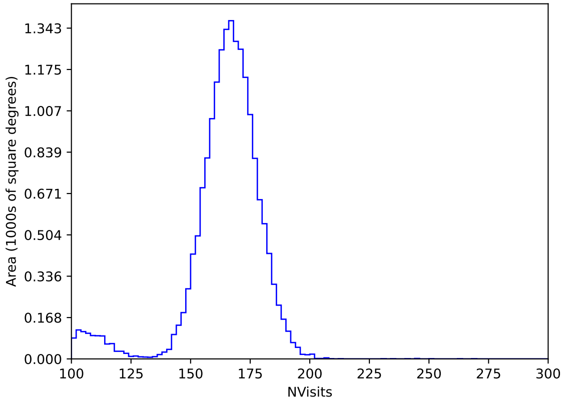
too_elab_r64_d3_giz_v3.4_10yrs WFD y band: NVisits
