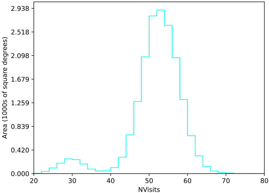
too_elab_r64_d3_giz_v3.4_10yrs WFD u band: NVisits
