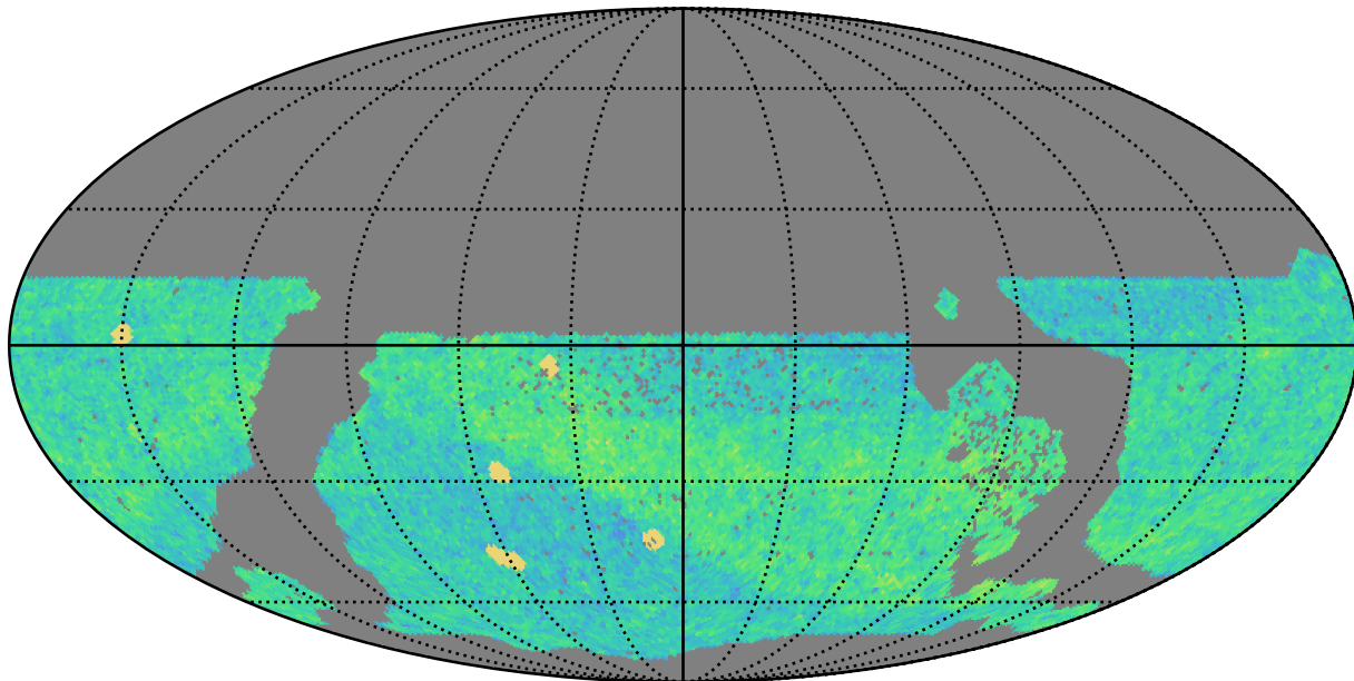
too_elab_r64_d3_giz_v3.4_10yrs WFD i band: NVisits
