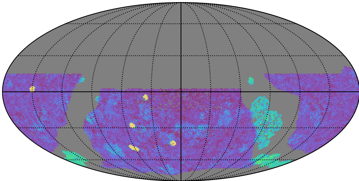
too_elab_r64_d3_giz_v3.4_10yrs WFD g band: NVisits
