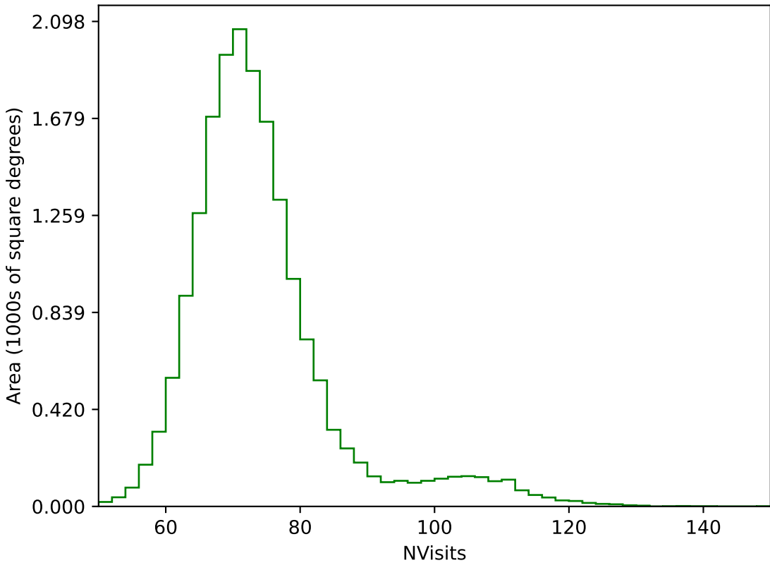
too_elab_r64_d3_giz_v3.4_10yrs WFD g band: NVisits
