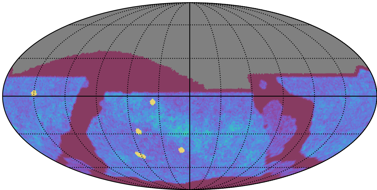
too_elab_r64_d3_giz_v3.4_10yrs All sky z band: NVisits
