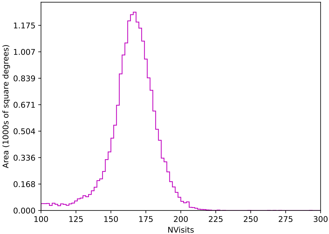
too_elab_r64_d3_giz_v3.4_10yrs All sky z band: NVisits
