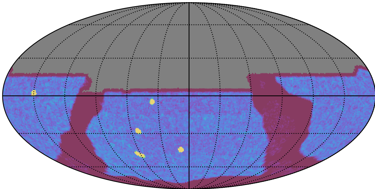
too_elab_r64_d3_giz_v3.4_10yrs All sky y band: NVisits
