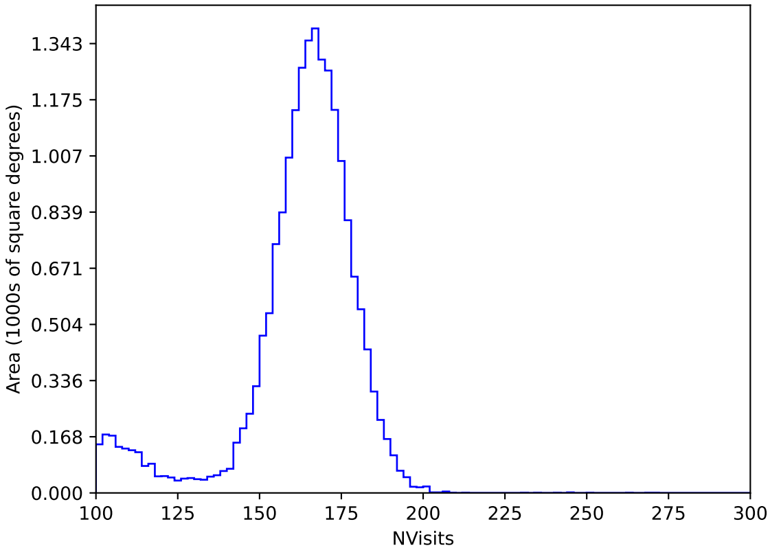
too_elab_r64_d3_giz_v3.4_10yrs All sky y band: NVisits
