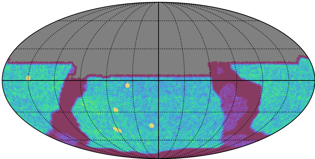
too_elab_r64_d3_giz_v3.4_10yrs All sky u band: NVisits
