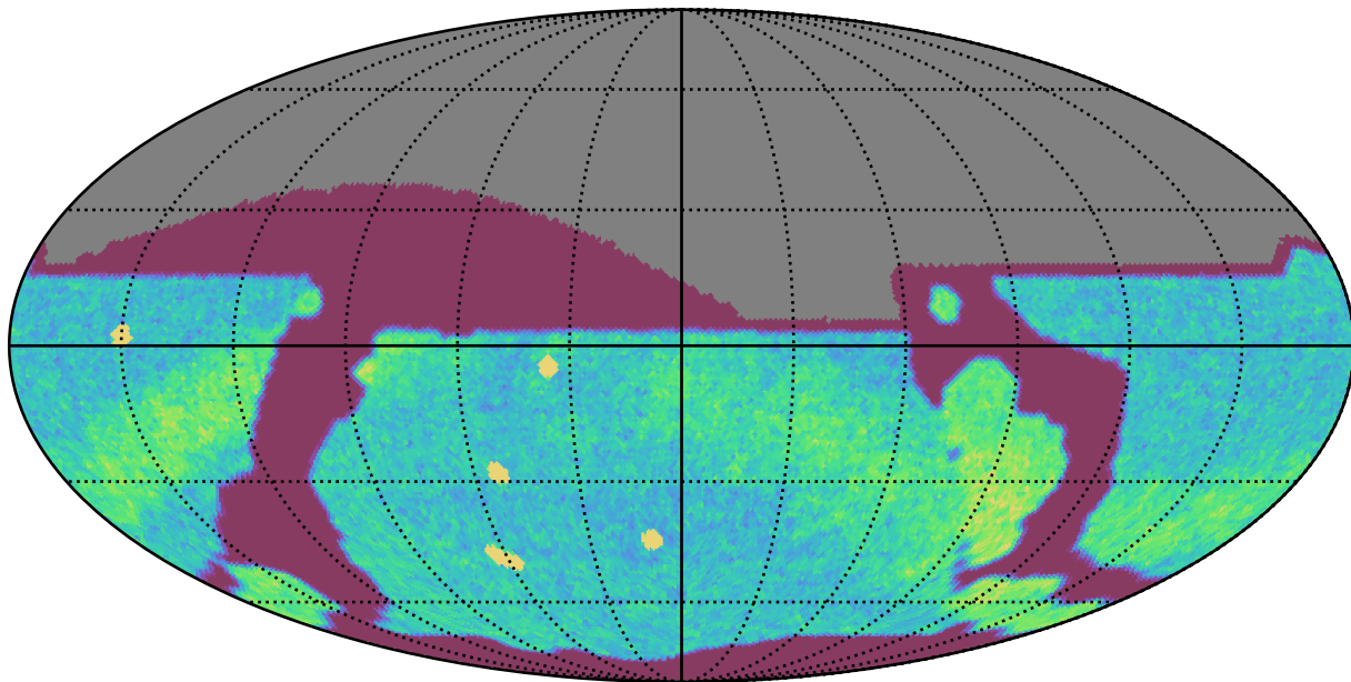
too_elab_r64_d3_giz_v3.4_10yrs All sky r band: NVisits
